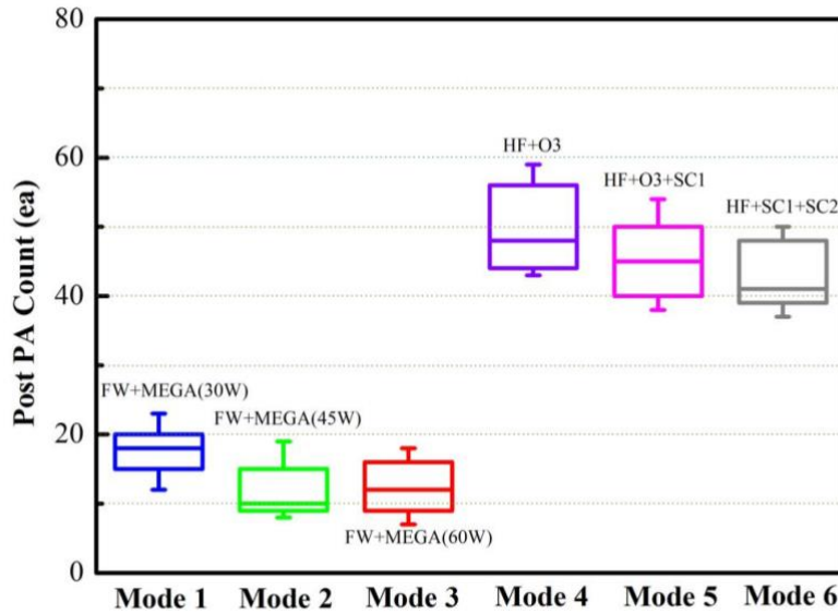
Fig. 4: Comparison of six clean mode (Mode1-Mode 6) to surface PA remove ability
